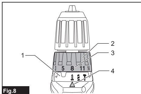
Fig.8 ► 1. Action mode changing ring 2. Adjusting ring 3. Graduation 4. Arrow
