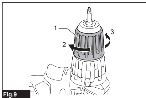
Fig.9 ► 1. Sleeve 2. Close 3. Open
